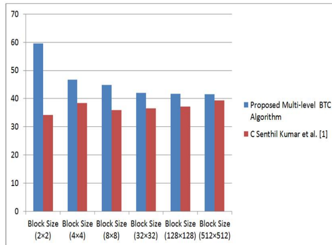
Figure 6: MSE for Different Block Size using Satellite Image
