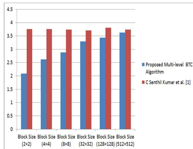
Figure 7: Computation Time for Different Block Size using Satellite Image
