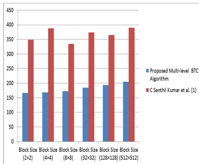
Figure 5: MSE for Different Block Size using Satellite Image
