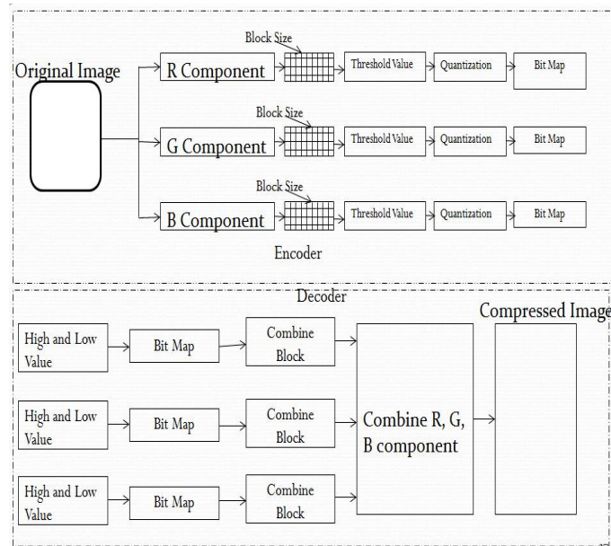
Figure 2: Block Diagram of Proposed Algorithm
